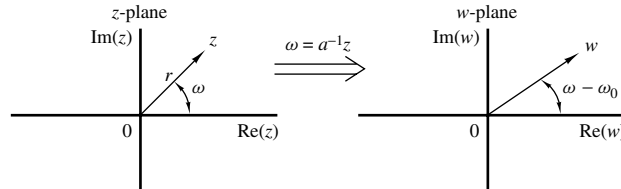
Figure 2.1 Mapping of the z -plane to the w -plane via the transformation w = a^{-1}z , a = r_0 e^{j\omega_0} .
